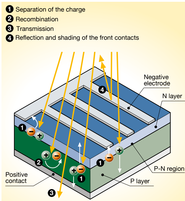
Figure 1.9 - Photovoltaic effect
