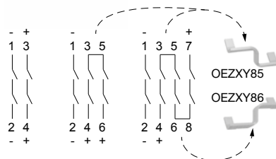
Wiring diagram
