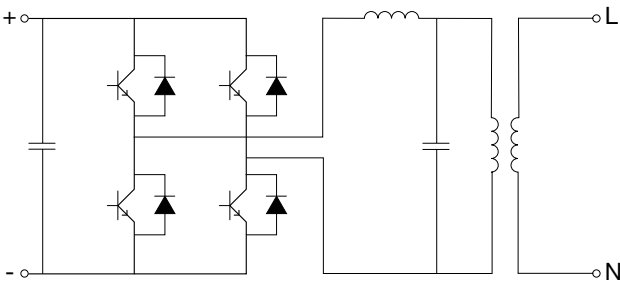
Figure 1.14 – Principle scheme of a single-phase inverter
